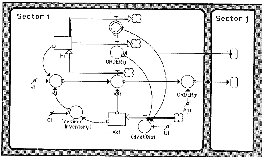
Figure 1: Stock-flow diagram
