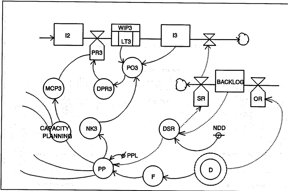
Figure 1. The kanban system model.
